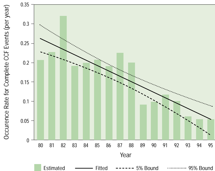
Figure 1 Evolution of the frequency of common-cause failures over time [25].
