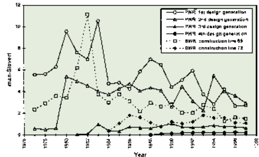
Figure 4: Mean annual collective doses of nuclear power plants per year and plant [7]
