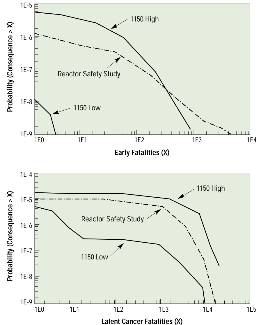
Figure 3 Comparison of the cumulative frequency of occurrence damage function between NUREG-1150 and RSS (Wash-1400)
