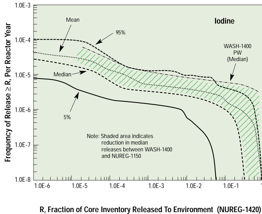
Figure 2 Frequency of Exceeding Iodine Release Fractions in NUREG-1150 and RSS (Wash-1400) Analysis of Surry, [26]
